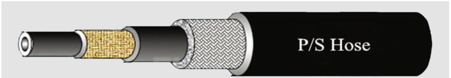
Tube Reinforcement Buffer with Reinforcement Cover
